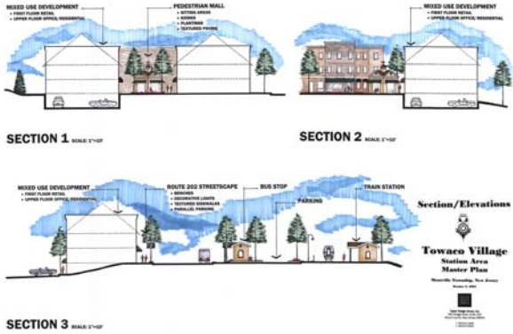
SECTION 1 SCALE 1"=100' SECTION 2 SCALE 1"=100' SECTION 3 SCALE 1"=100' Elevation Graphics
